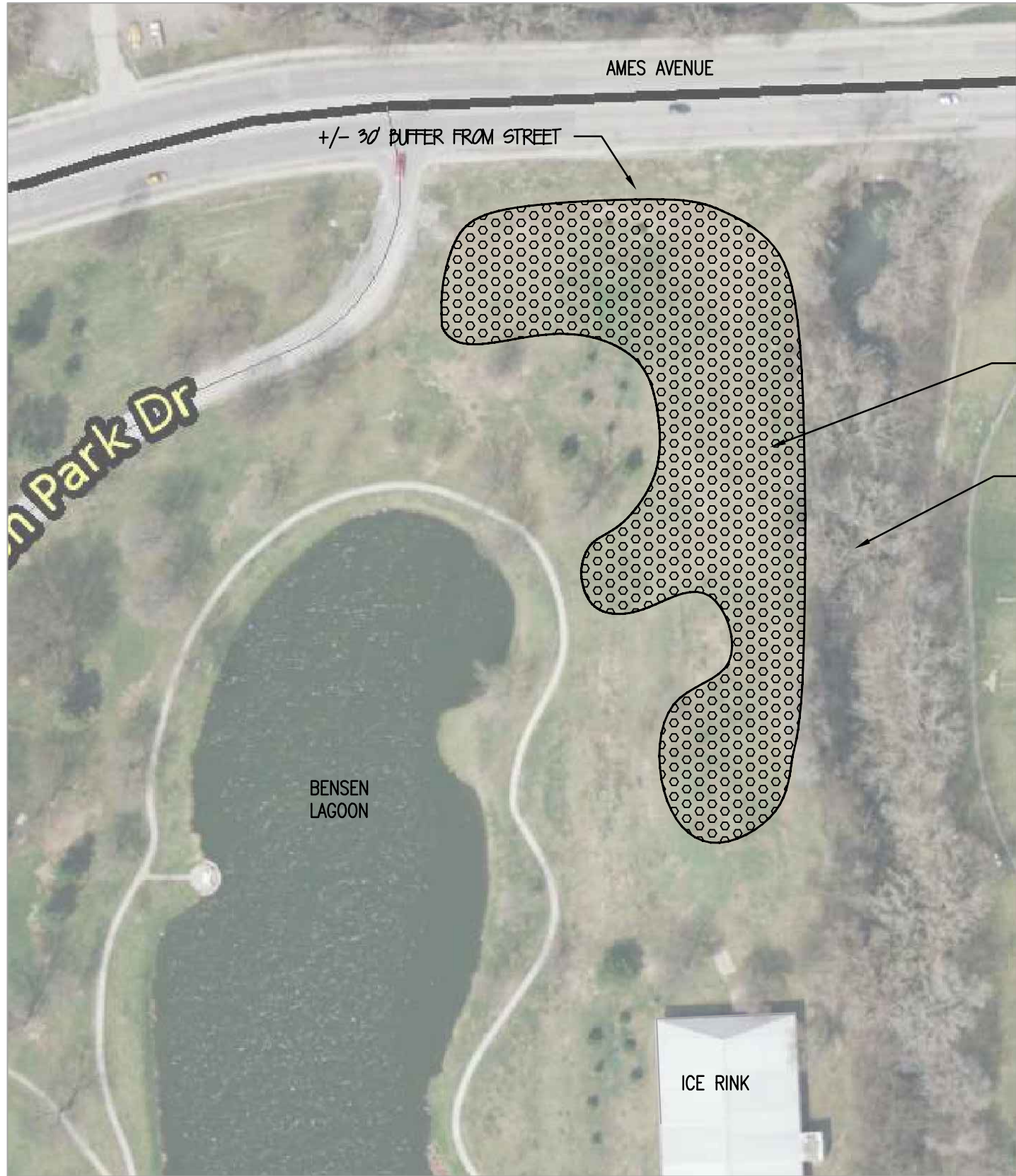
PHASE I PRAIRIE LAYOUT SCALE: 1" = 100'-0"
